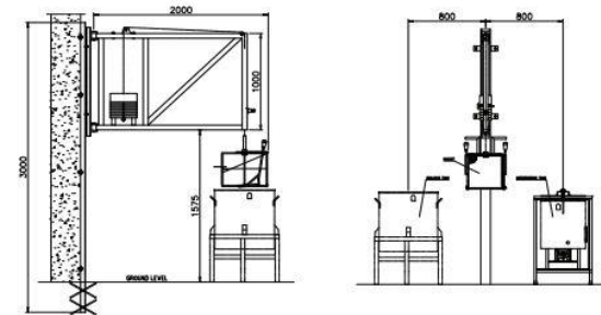
12 Killing Cones
